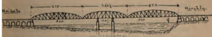
SKETCH DIAGRAM OF HOOGHLY BRIDGE.
