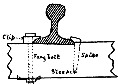
FLAT-FOOTED RAIL.
